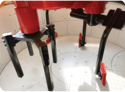
快速搅拌叶片 High Speed Mixing Blade
